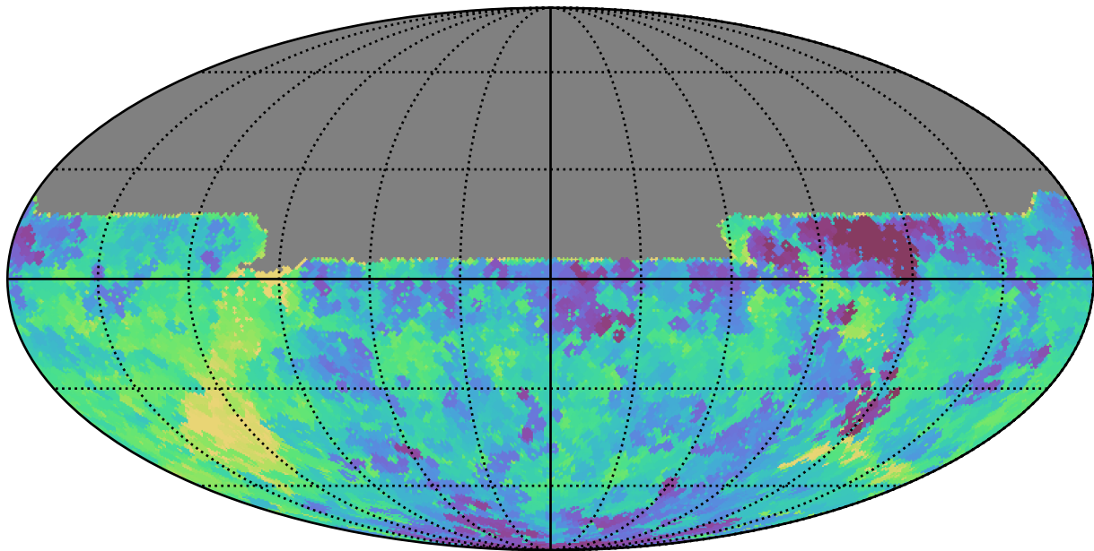
too_100_1v3.4_10yrs All sky u band: Min saturation_mag
