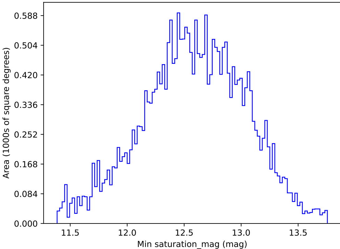
too_100_1v3.4_10yrs All sky r band: Min saturation_mag
