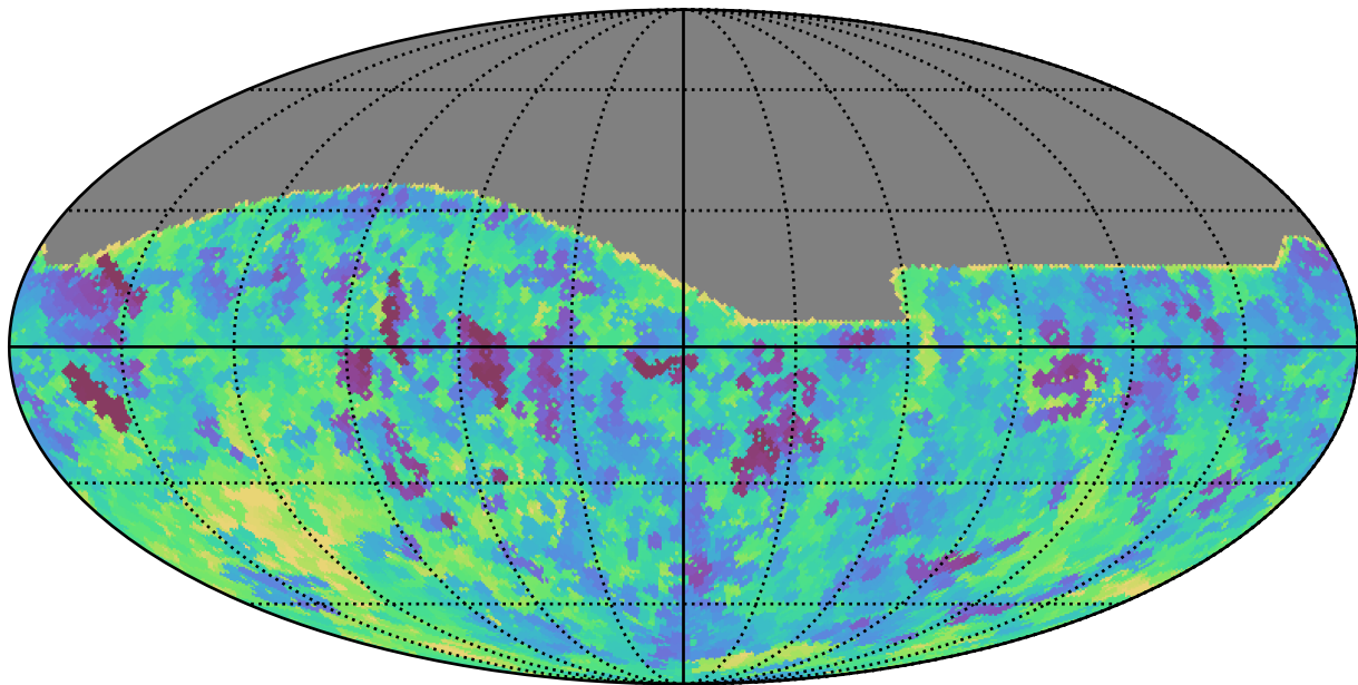
too_100_1v3.4_10yrs All sky i band: Min saturation_mag
