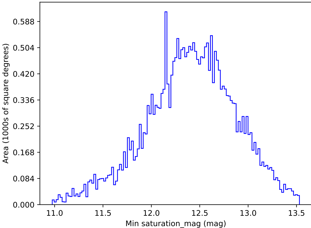
too_100_1v3.4_10yrs All sky i band: Min saturation_mag
