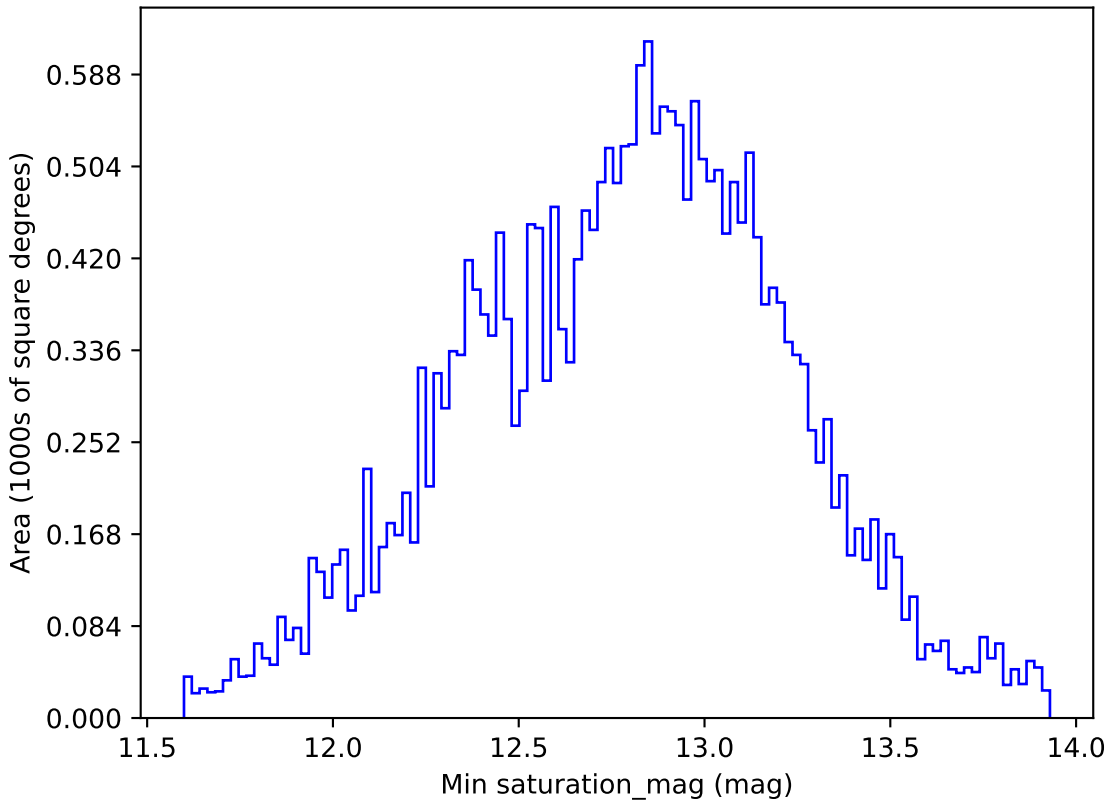
too_100_1v3.4_10yrs All sky g band: Min saturation_mag
