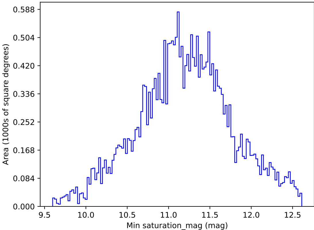
too_100_1v3.4_10yrs All sky all bands: Min saturation_mag
