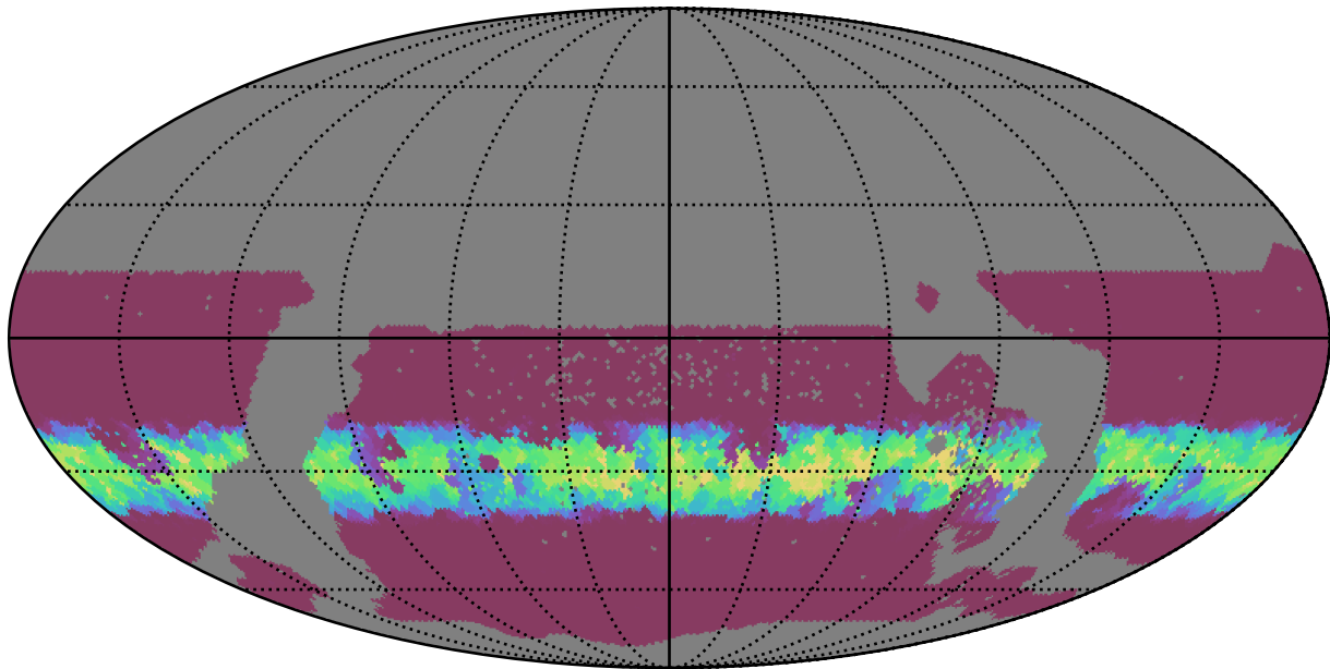
too_100_1v3.4_10yrs WFD z band: Min normairmass
