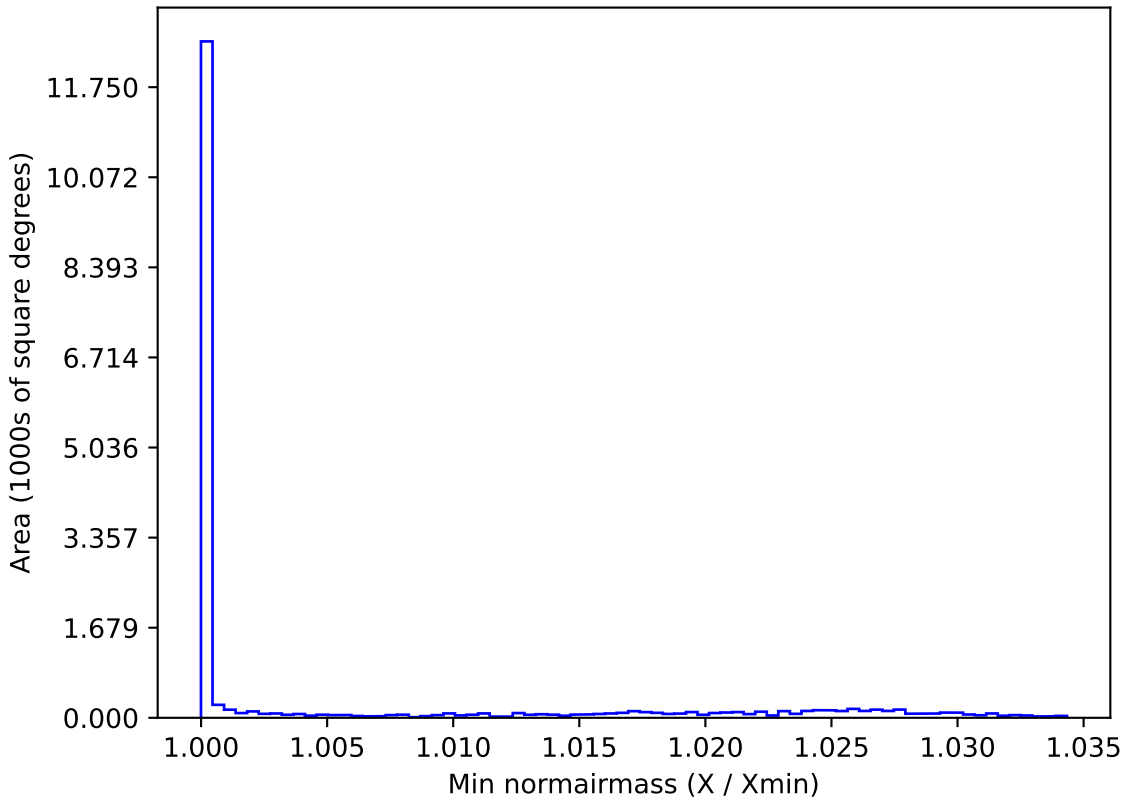
too_100_1v3.4_10yrs WFD z band: Min normairmass
