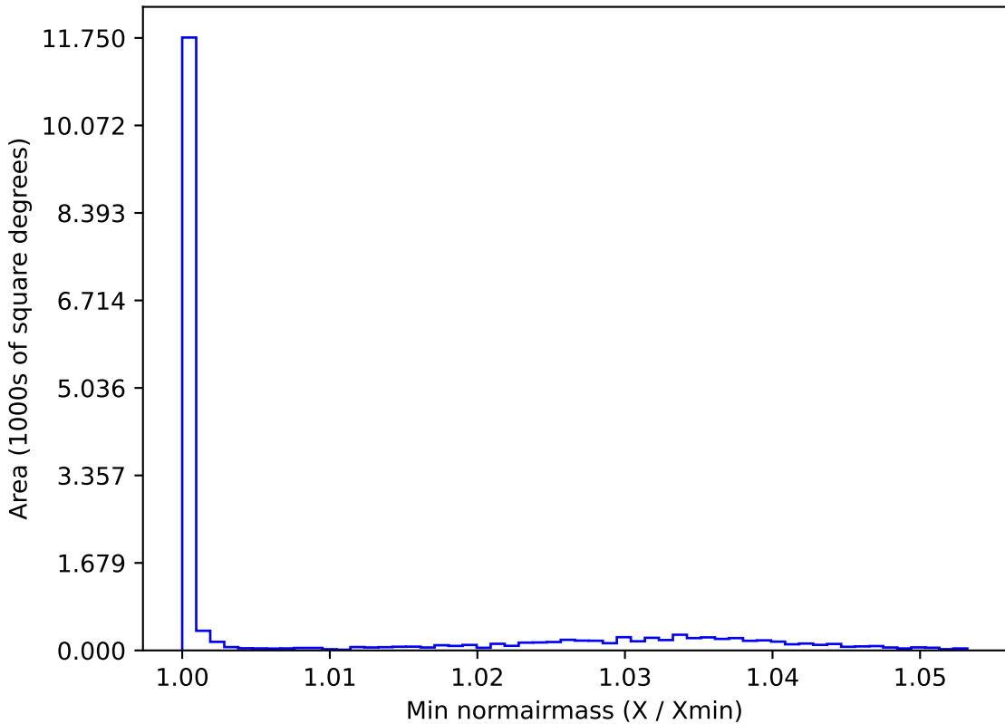
too_100_1v3.4_10yrs WFD u band: Min normairmass
