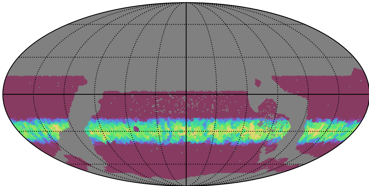
too_100_1v3.4_10yrs WFD i band: Min normairmass
