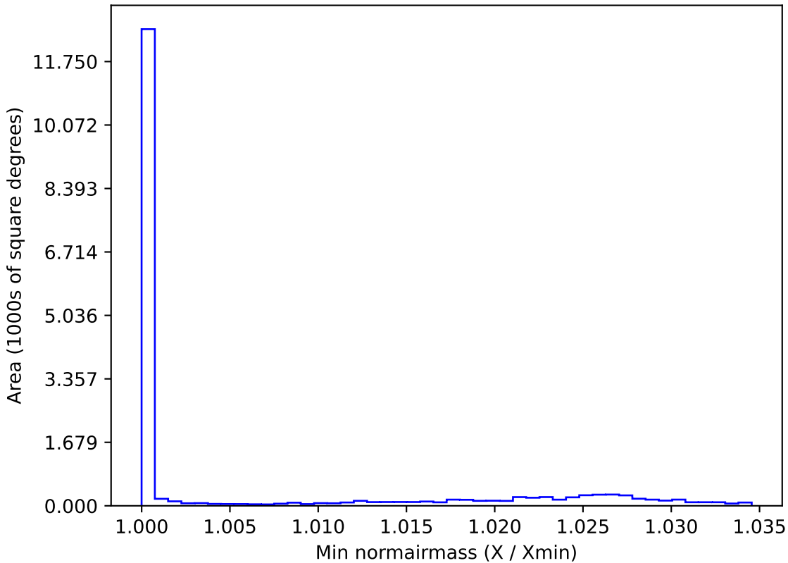
too_100_1v3.4_10yrs WFD i band: Min normairmass
