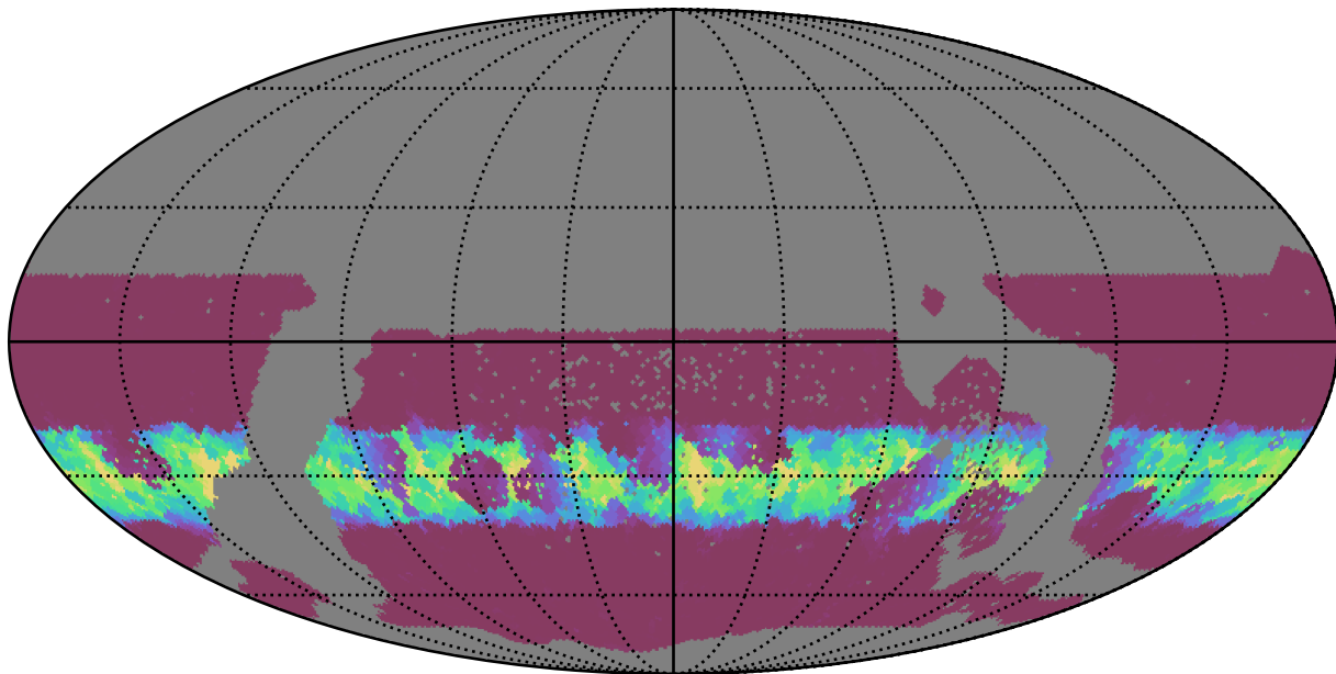
too_100_1v3.4_10yrs WFD g band: Min normairmass
