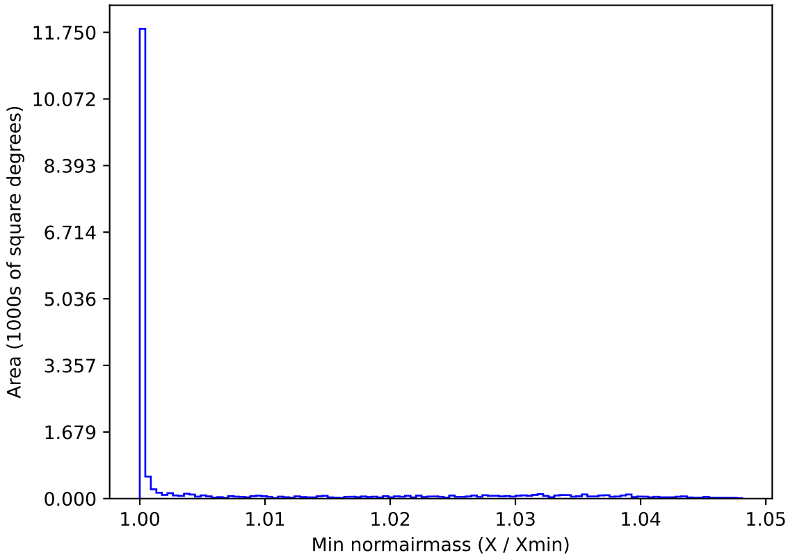
too_100_1v3.4_10yrs WFD g band: Min normairmass
