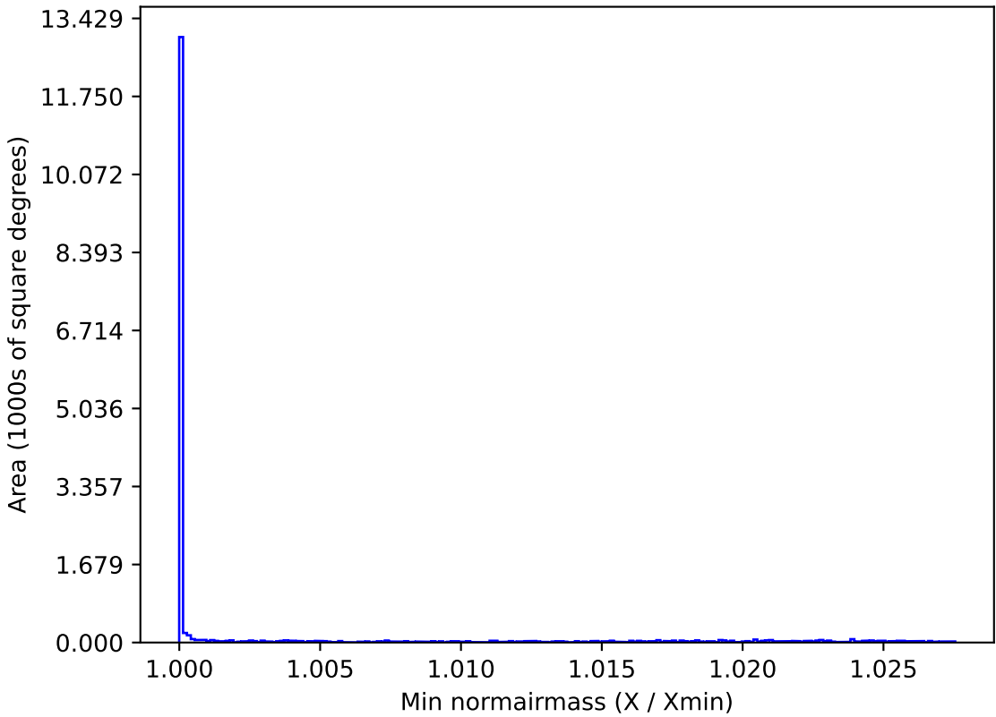
too_100_1v3.4_10yrs WFD all bands: Min normairmass
