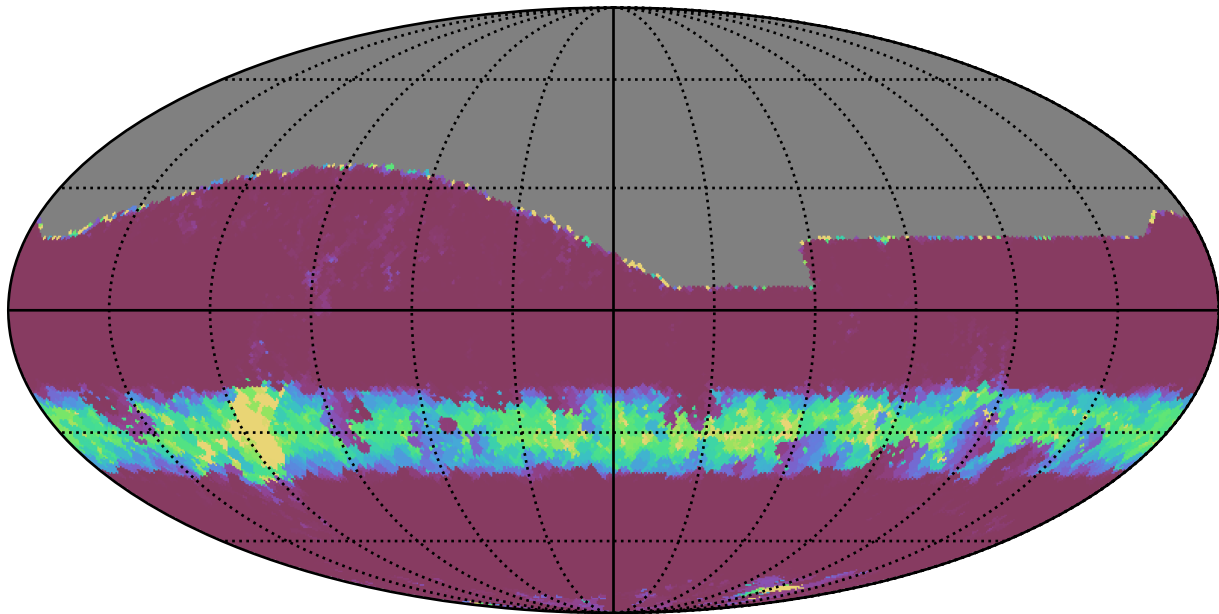
too_100_1v3.4_10yrs All sky z band: Min normairmass
