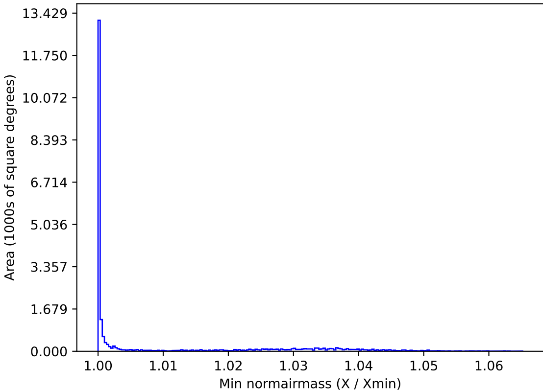
too_100_1v3.4_10yrs All sky u band: Min normairmass
