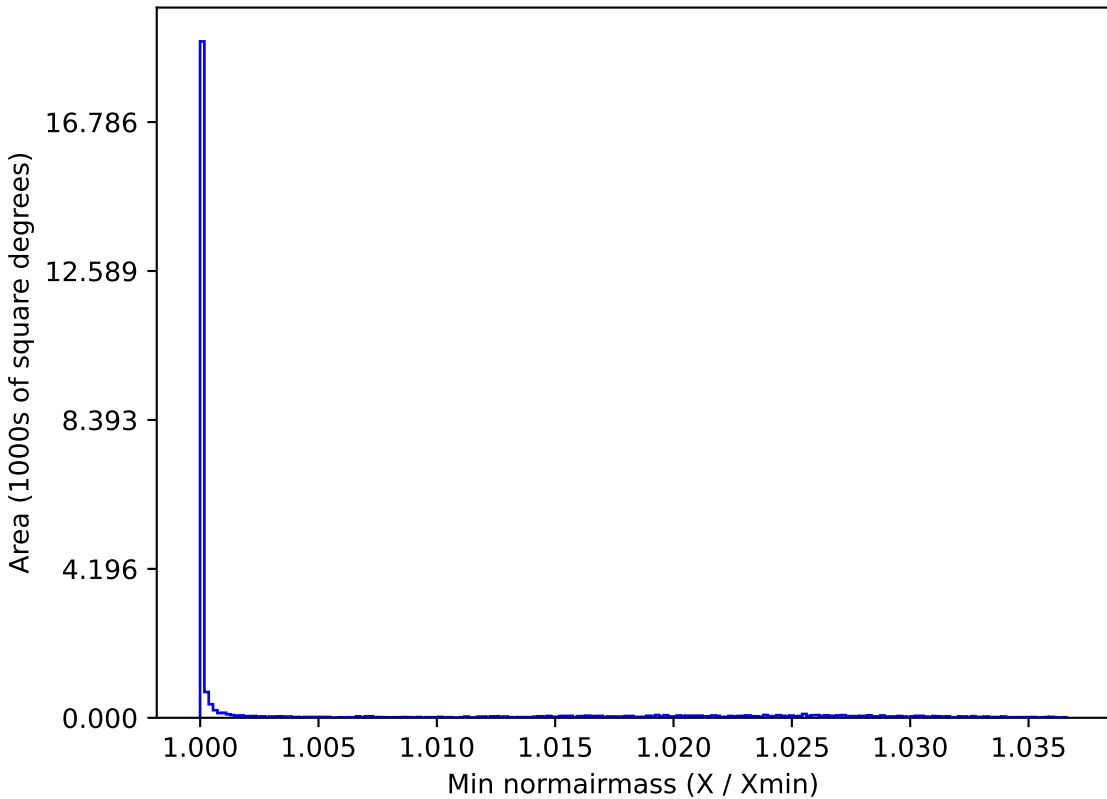
too_100_1v3.4_10yrs All sky r band: Min normairmass
