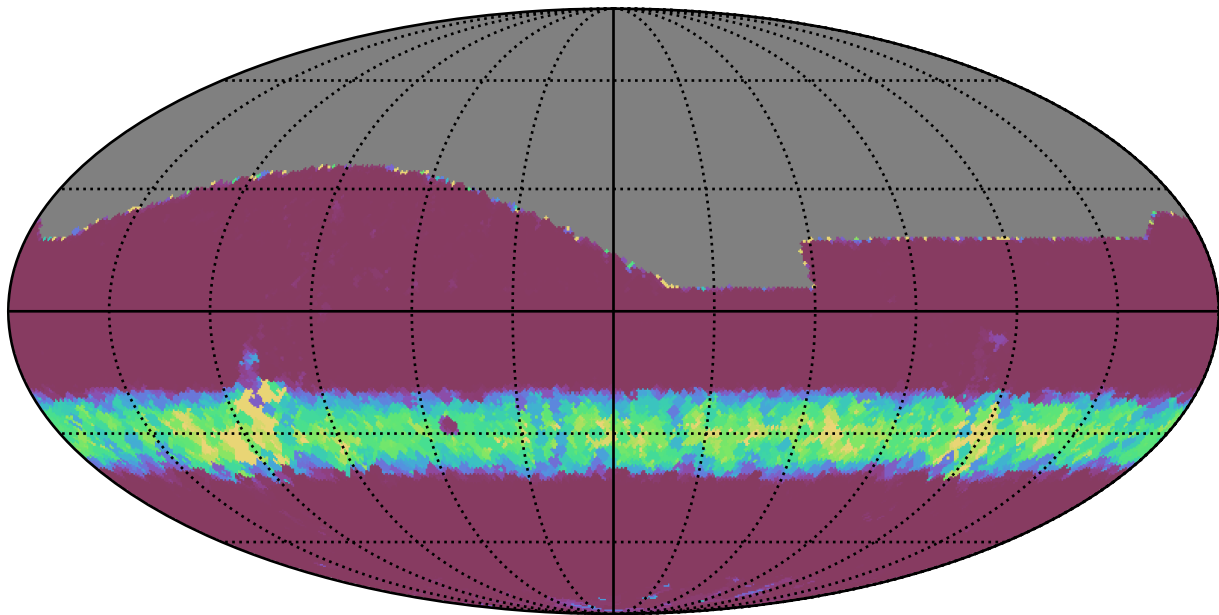
too_100_1v3.4_10yrs All sky i band: Min normairmass
