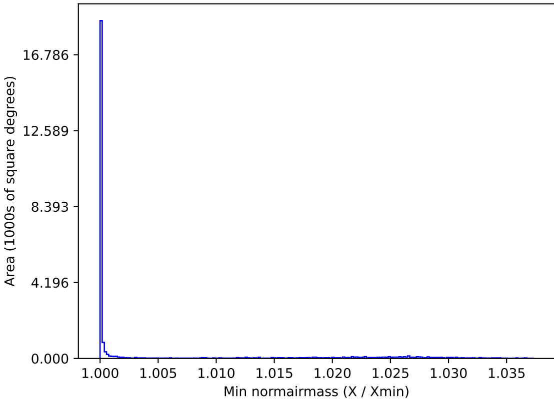
too_100_1v3.4_10yrs All sky i band: Min normairmass
