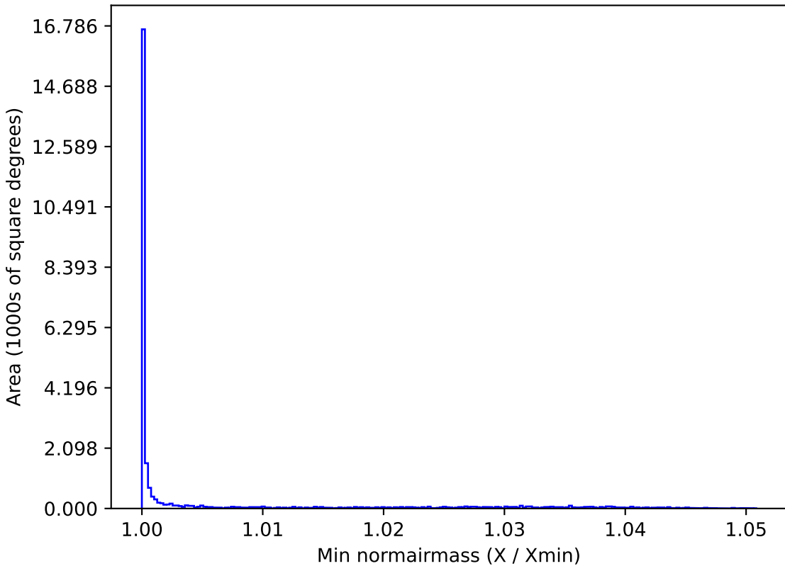
too_100_1v3.4_10yrs All sky g band: Min normairmass
