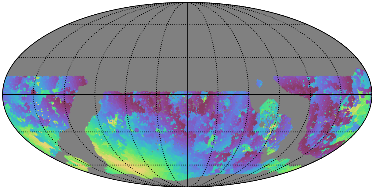
too_100_1v3.4_10yrs WFD u band: Min moonDistance
