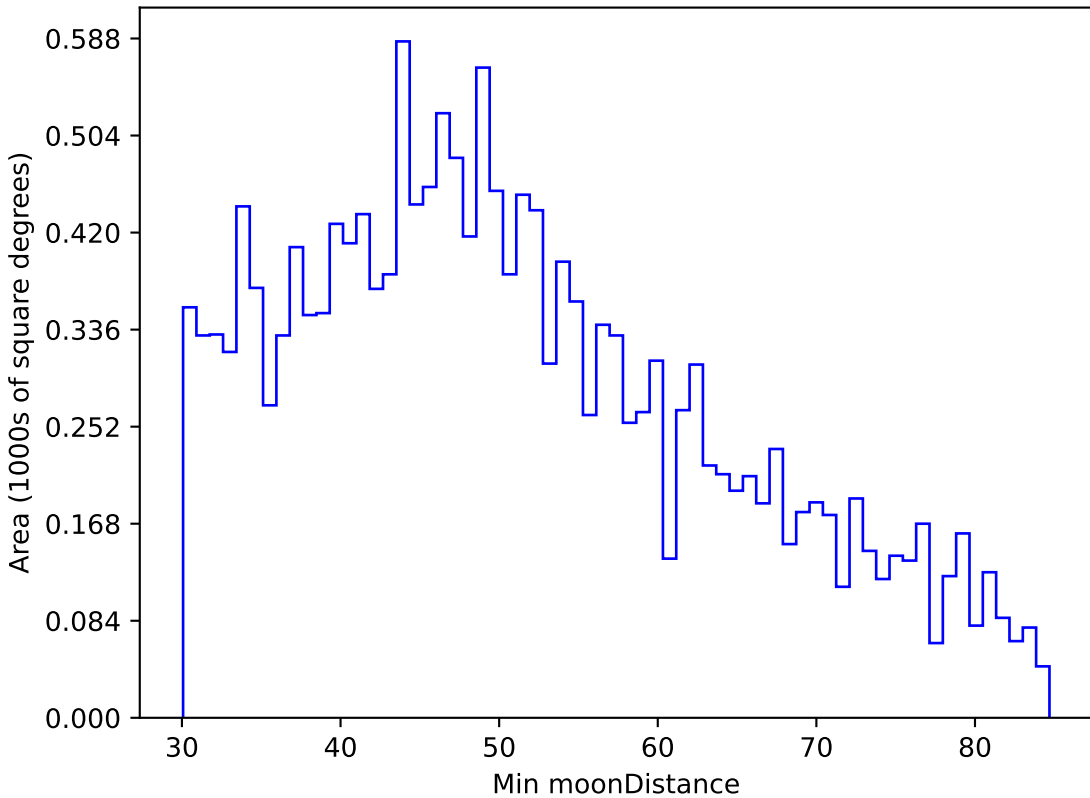
too_100_1v3.4_10yrs WFD u band: Min moonDistance
