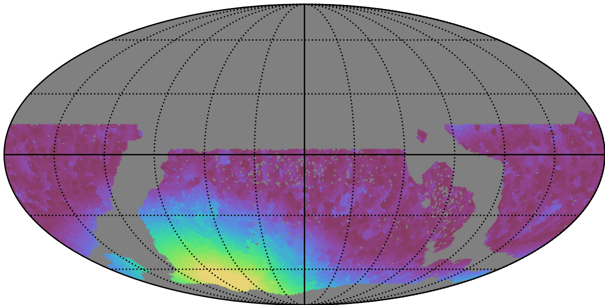
too_100_1v3.4_10yrs WFD r band: Min moonDistance
