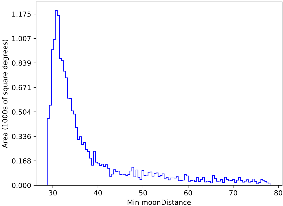
too_100_1v3.4_10yrs WFD r band: Min moonDistance
