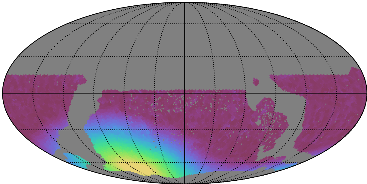
too_100_1v3.4_10yrs WFD i band: Min moonDistance
