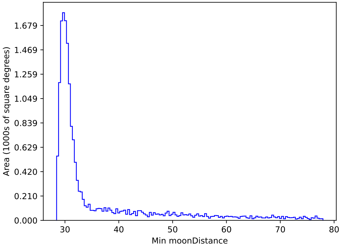
too_100_1v3.4_10yrs WFD i band: Min moonDistance
