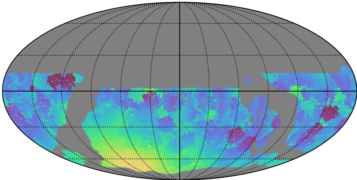
too_100_1v3.4_10yrs WFD g band: Min moonDistance
