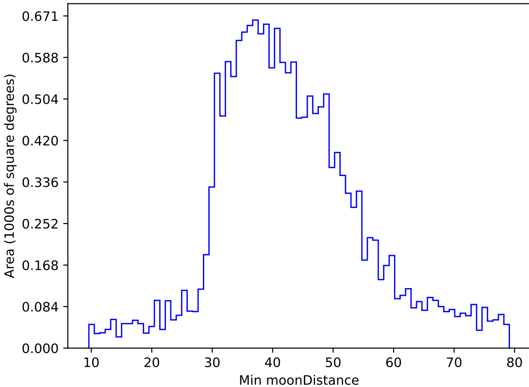
too_100_1v3.4_10yrs WFD g band: Min moonDistance
