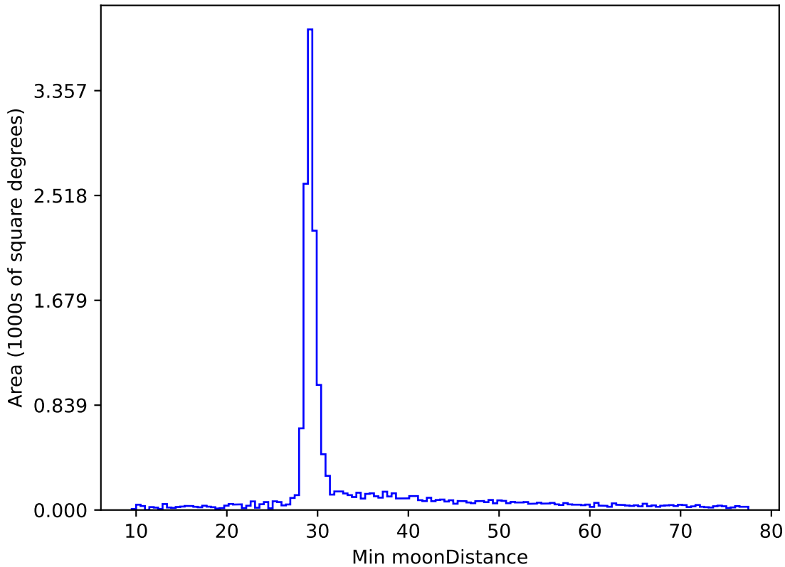
too_100_1v3.4_10yrs WFD all bands: Min moonDistance
