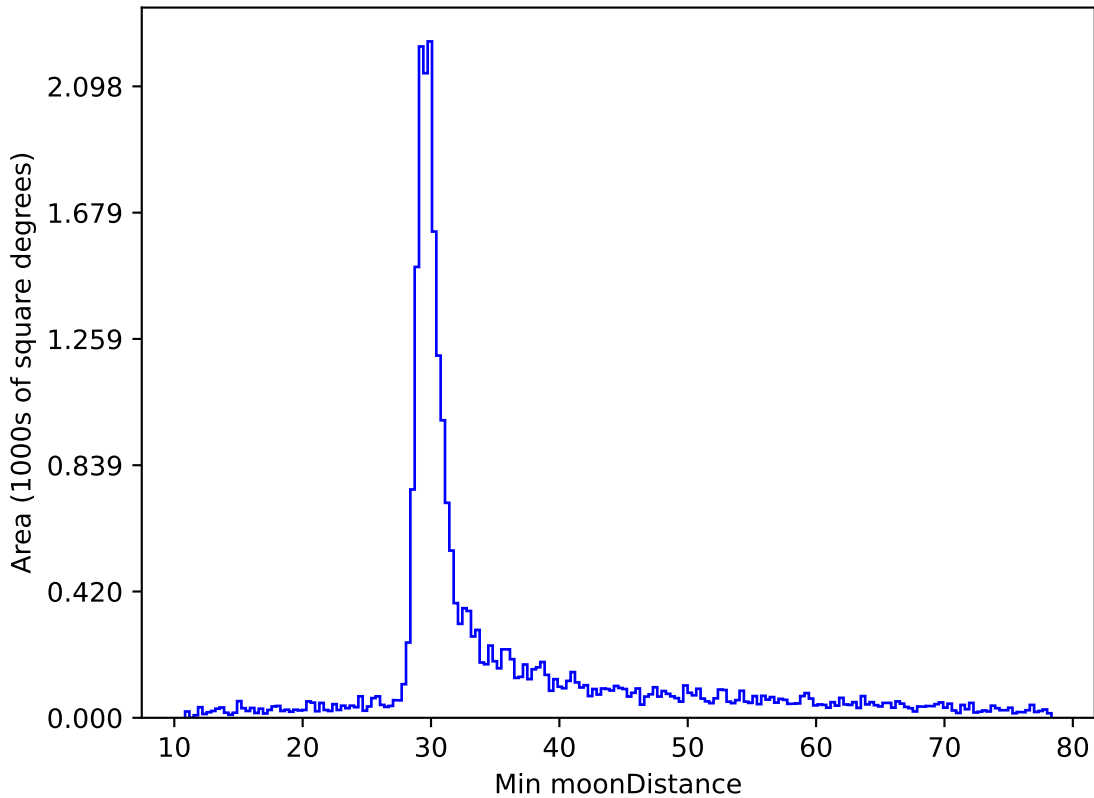
too_100_1v3.4_10yrs All sky z band: Min moonDistance
