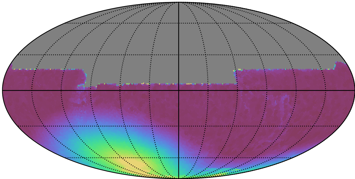
too_100_1v3.4_10yrs All sky y band: Min moonDistance
