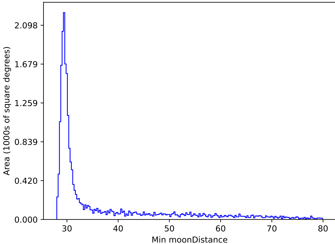
too_100_1v3.4_10yrs All sky y band: Min moonDistance
