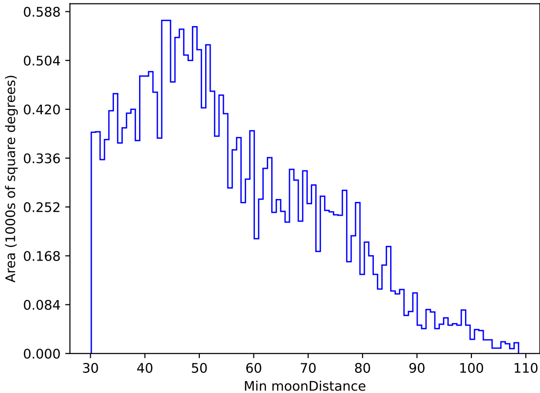
too_100_1v3.4_10yrs All sky u band: Min moonDistance
