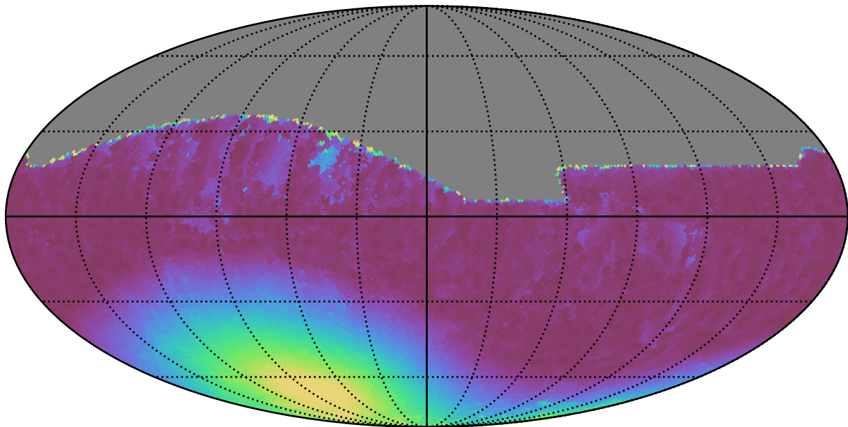
too_100_1v3.4_10yrs All sky i band: Min moonDistance
