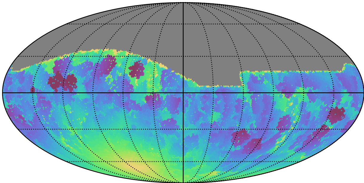
too_100_1v3.4_10yrs All sky g band: Min moonDistance
