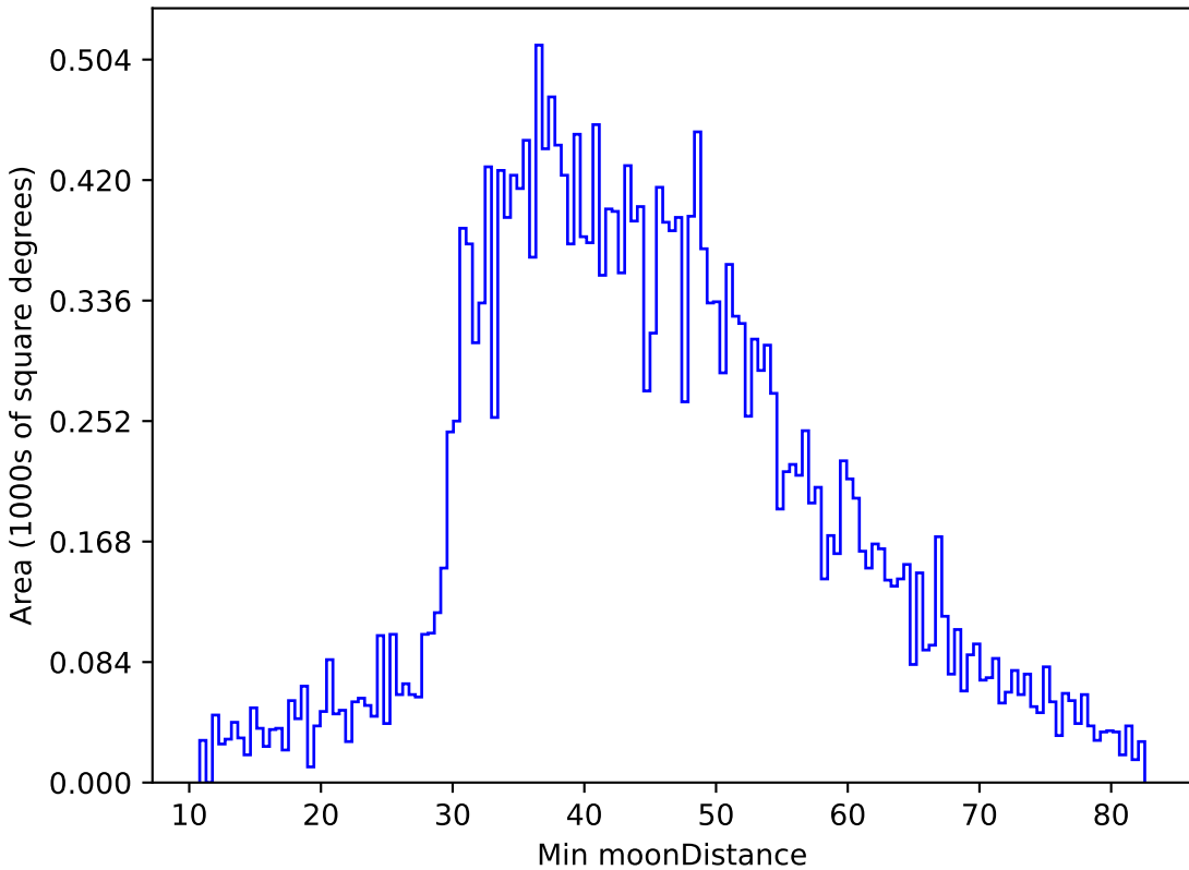
too_100_1v3.4_10yrs All sky g band: Min moonDistance
