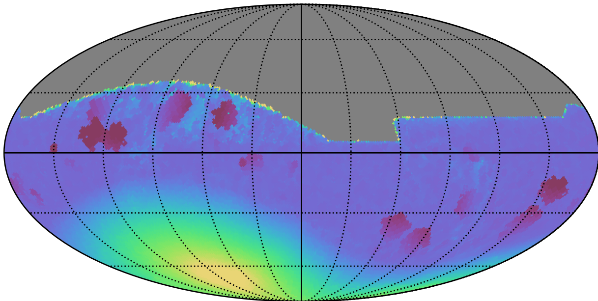
too_100_1v3.4_10yrs All sky all bands: Min moonDistance
