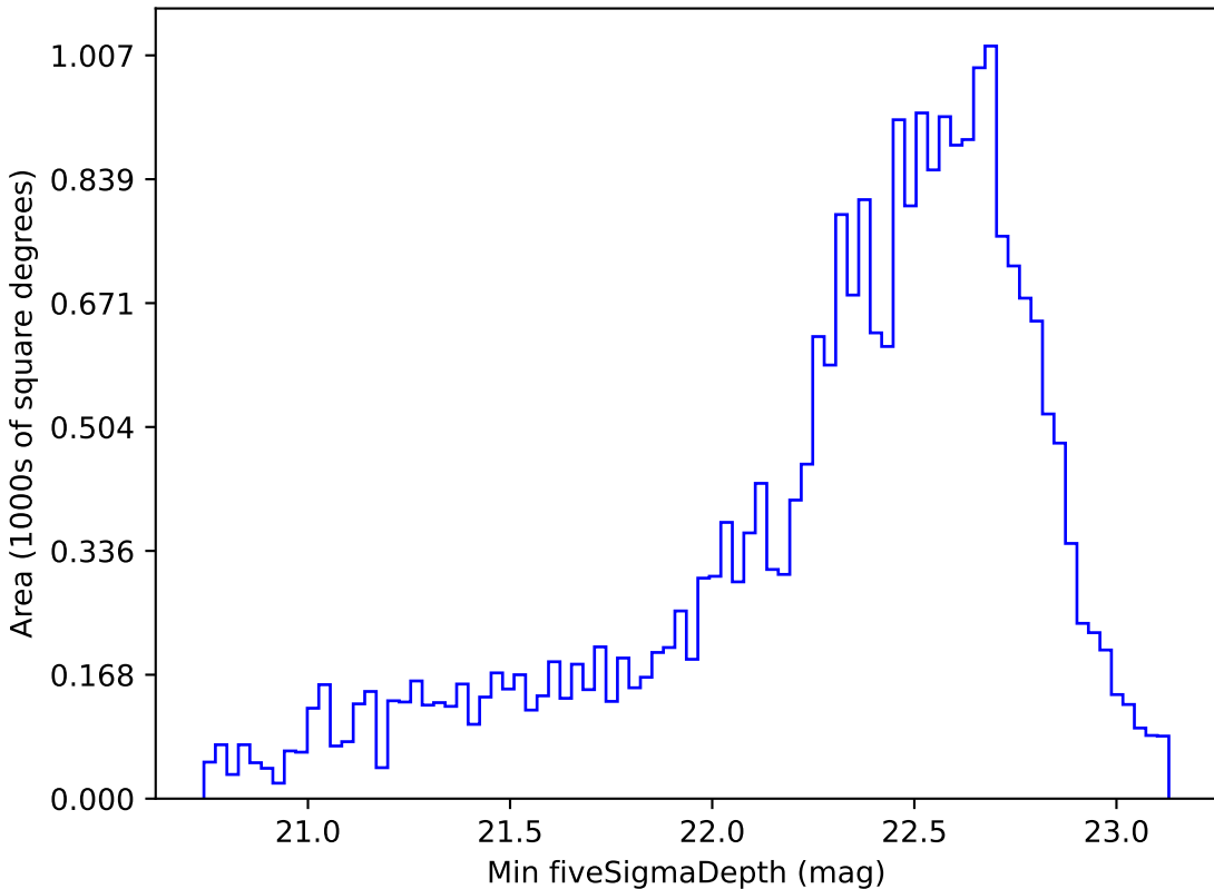
too_100_1v3.4_10yrs Yr 1 z band: Min fiveSigmaDepth
