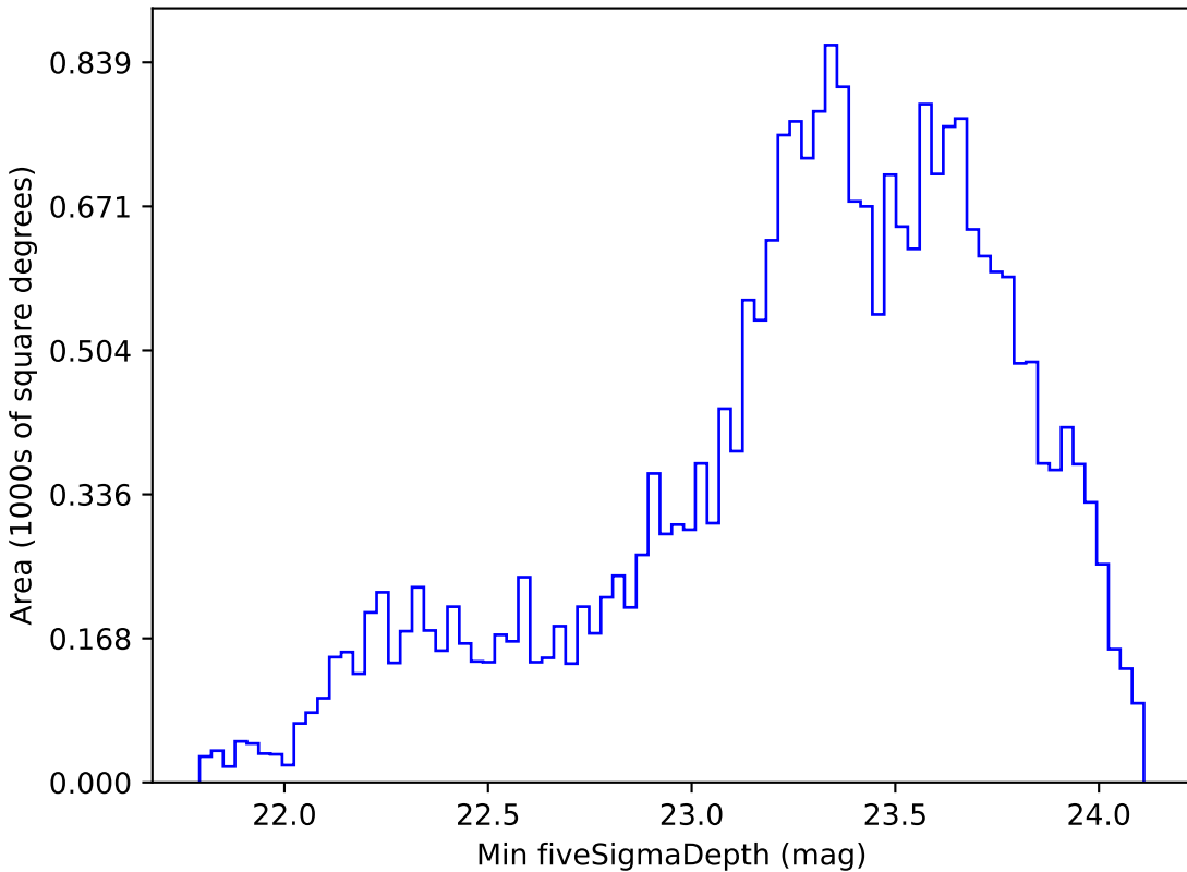
too_100_1v3.4_10yrs Yr 1 r band: Min fiveSigmaDepth
