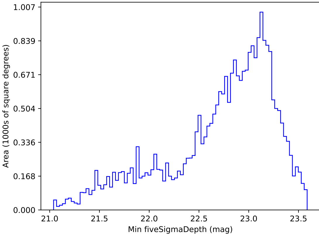
too_100_1v3.4_10yrs Yr 1 i band: Min fiveSigmaDepth
