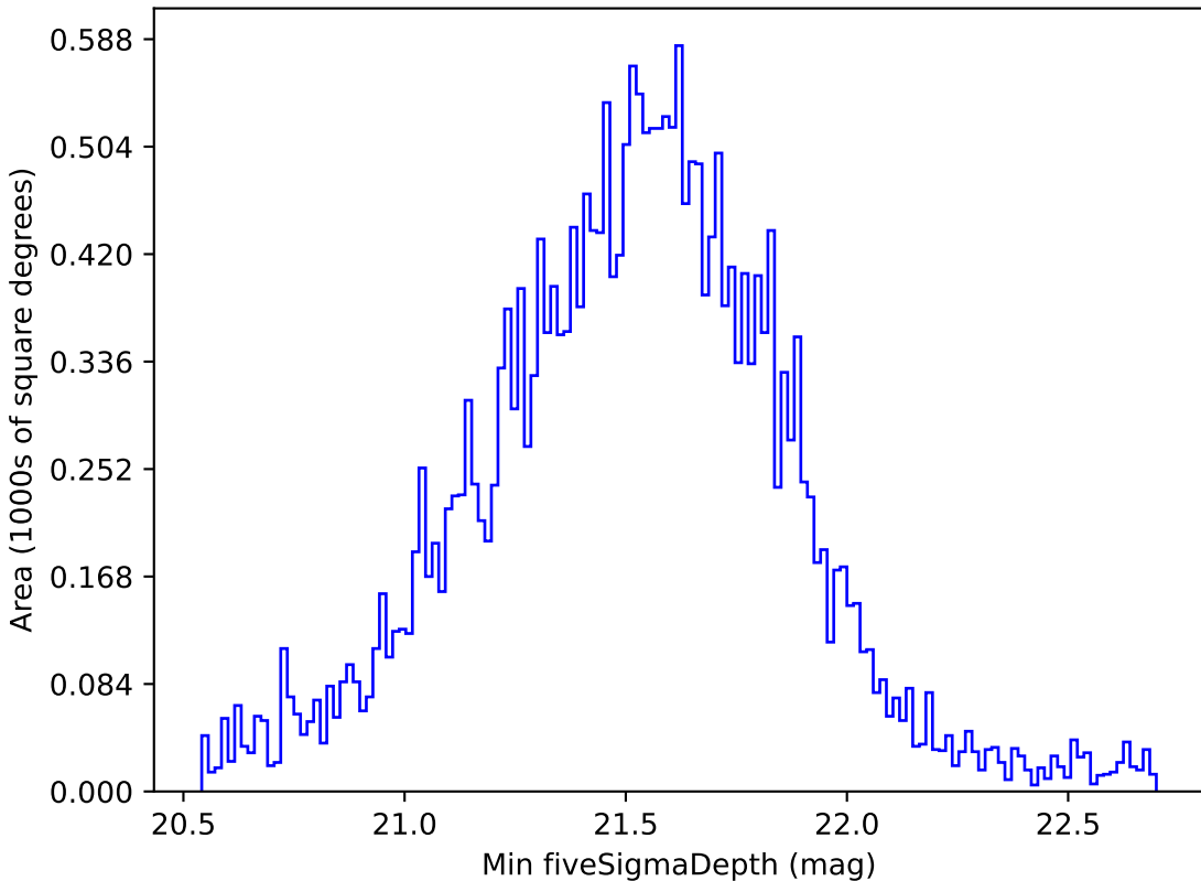
too_100_1v3.4_10yrs Yr 1 all bands: Min fiveSigmaDepth
