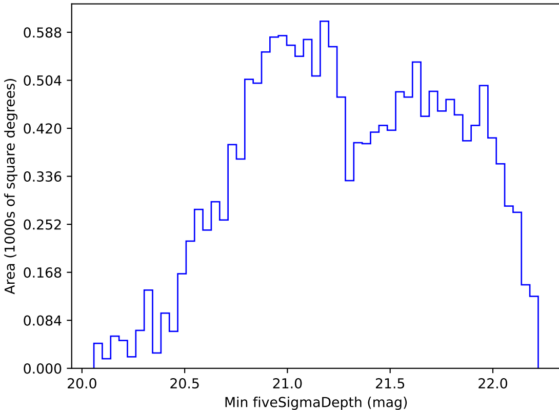
too_100_1v3.4_10yrs WFD z band: Min fiveSigmaDepth
