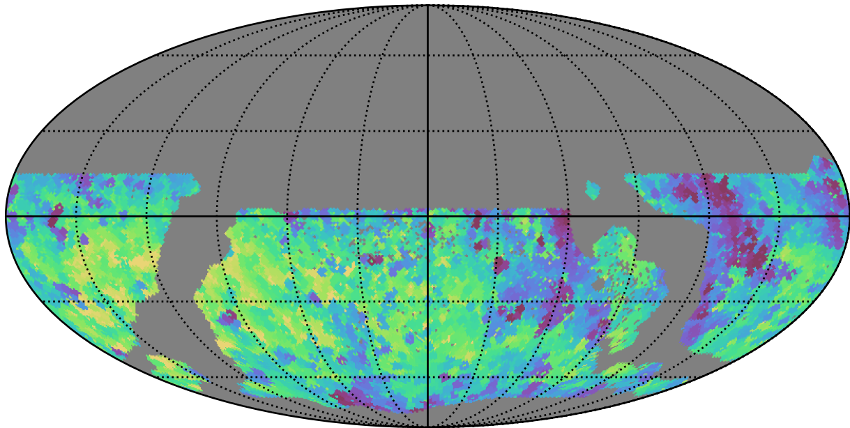
too_100_1v3.4_10yrs WFD y band: Min fiveSigmaDepth
