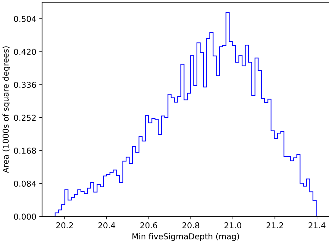
too_100_1v3.4_10yrs WFD y band: Min fiveSigmaDepth
