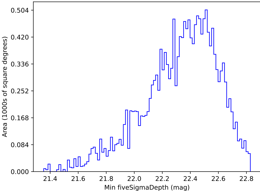
too_100_1v3.4_10yrs WFD u band: Min fiveSigmaDepth
