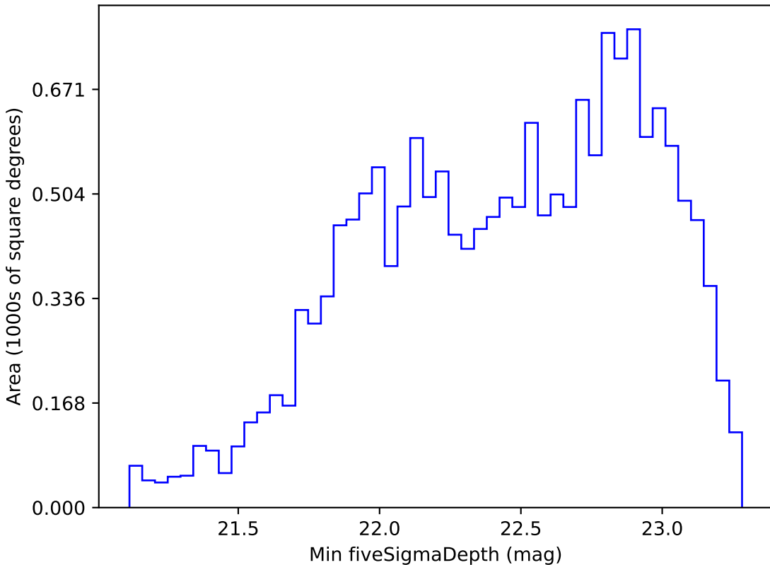
too_100_1v3.4_10yrs WFD r band: Min fiveSigmaDepth
