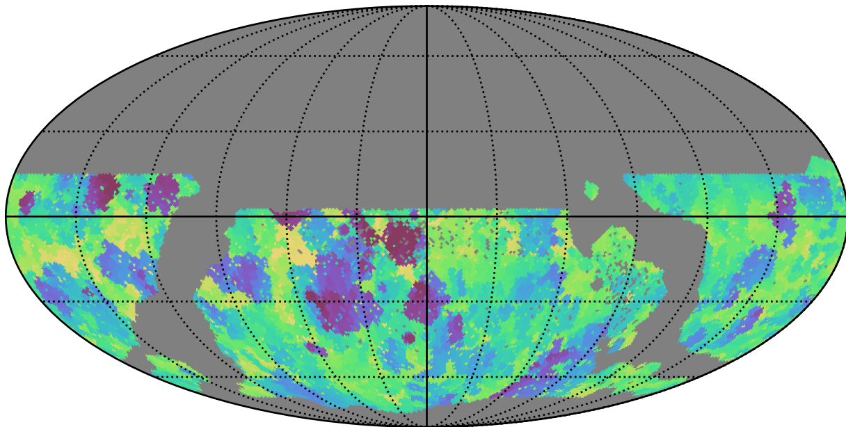
too_100_1v3.4_10yrs WFD g band: Min fiveSigmaDepth
