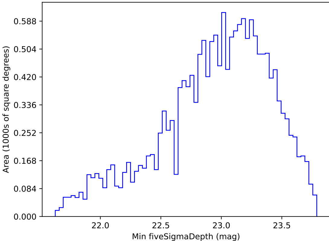
too_100_1v3.4_10yrs WFD g band: Min fiveSigmaDepth
