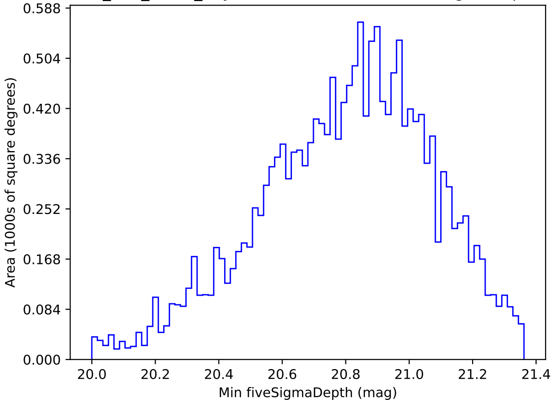
too_100_1v3.4_10yrs WFD all bands: Min fiveSigmaDepth
