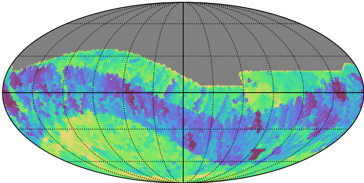
too_100_1v3.4_10yrs All sky z band: Min fiveSigmaDepth
